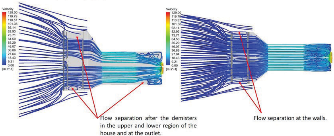
Streamlines in side (left) and top (right) view.
